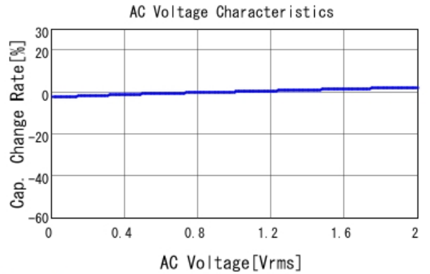
GRM188R72A104KA35 C-AC Voltage capchange, DCOV, 25
