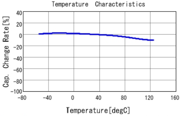
GRM188R72A104KA35 C-Temp. capchange, DC0.0V, AC1.C
