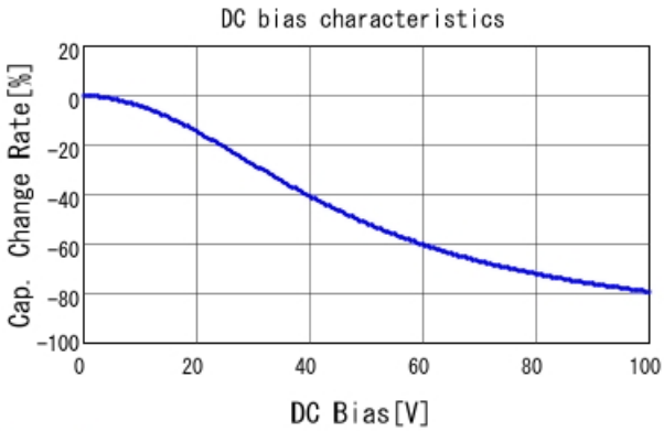
GRM188R72A104KA35 C-DC bias capchange, 25.0degC, A
